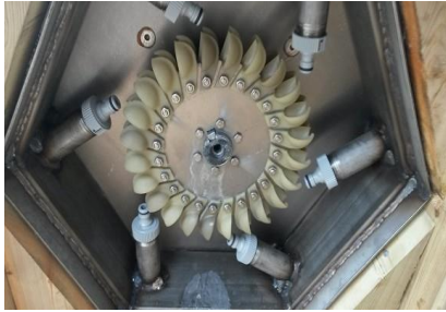
Pelton turbin 10 kW
